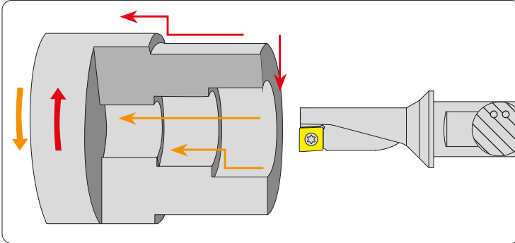
Delme Drilling Bohren
